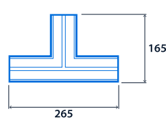
Tee Joint
